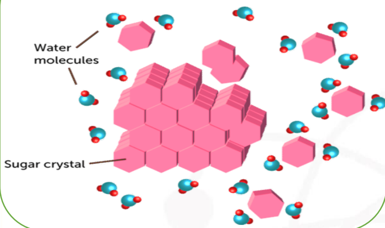
How Sugar Dissolves in Water
