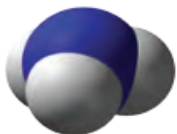
( \text{NH}_3 )
